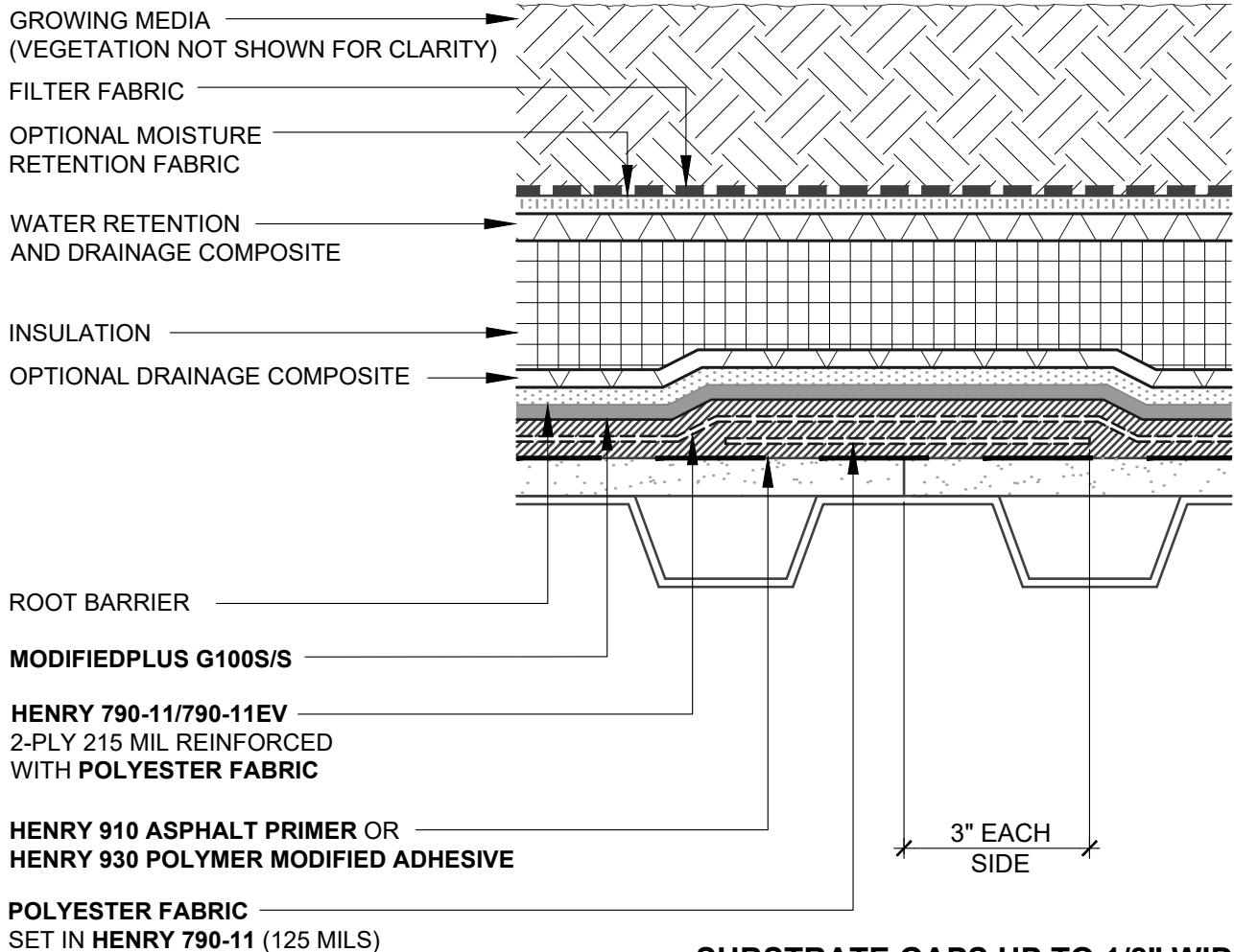
SUBSTRATE GAPS UP TO 1/8" WIDE N.T.S
